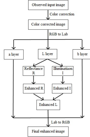
Fig. 1. The flow chart of the proposed algorithm.
